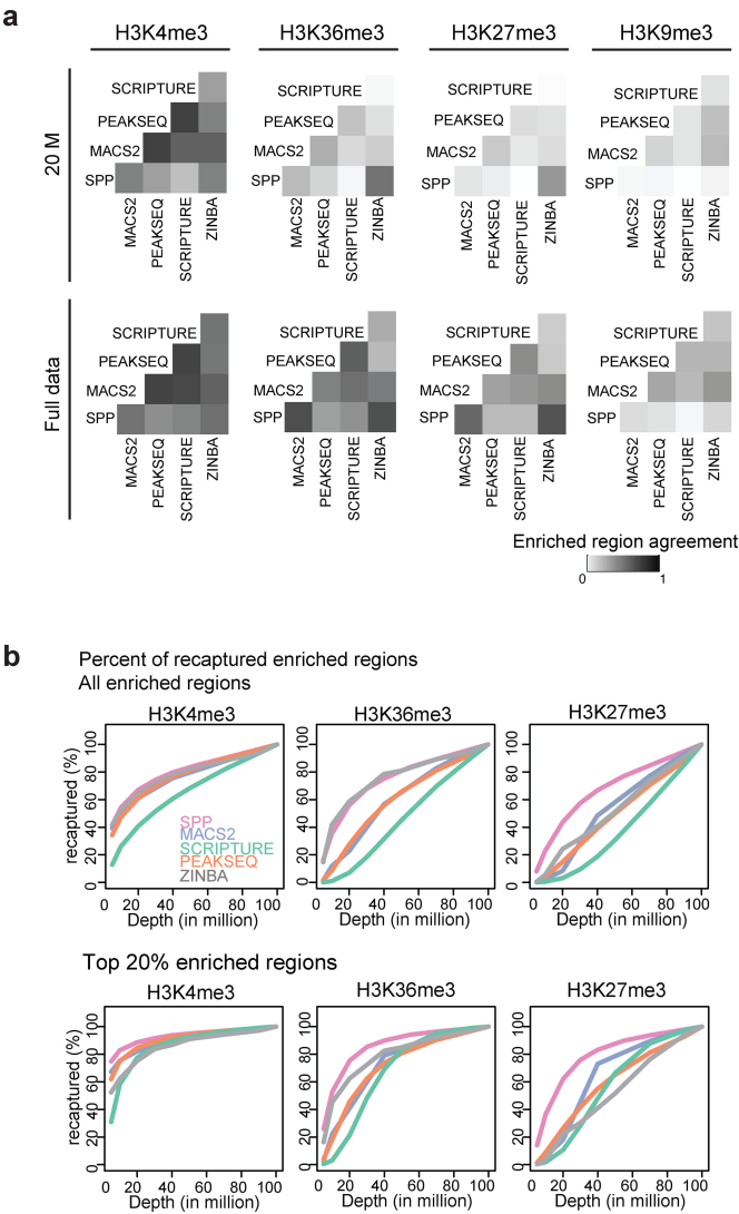
Figure 5. Comparison of enriched regions detected by various algorithms. (a) Each cell in the heatmaps shows the Jaccard similarity coefficient between the enriched regions (in bp) by each pair of methods at 20 million and 100 million reads for H3K4me3, H3K36me3 and H3K27me3, and at 20 million and 55 million reads for H3K9me3. (b) Percentage of the enriched regions recaptured at different sequencing depths for all regions (upper panels) and percentage of top 20% enriched regions recaptured at different sequencing depths (lower).
